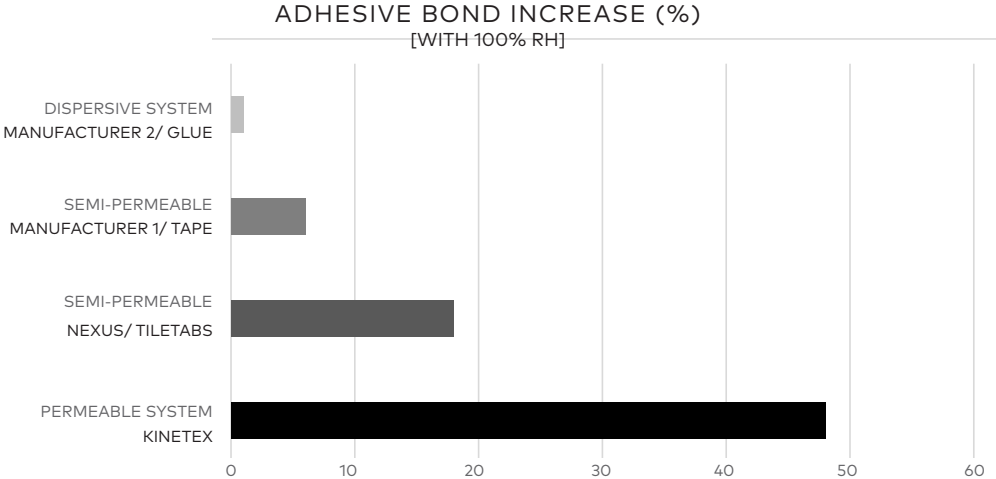
Figure 6. Adhesive Bond
