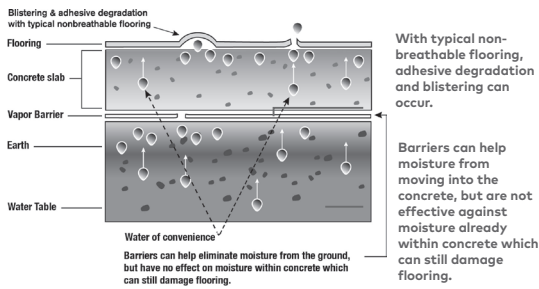
Figure 1. Moisture Activity Beneath and Within a Concrete Slab with Flooring Installed
